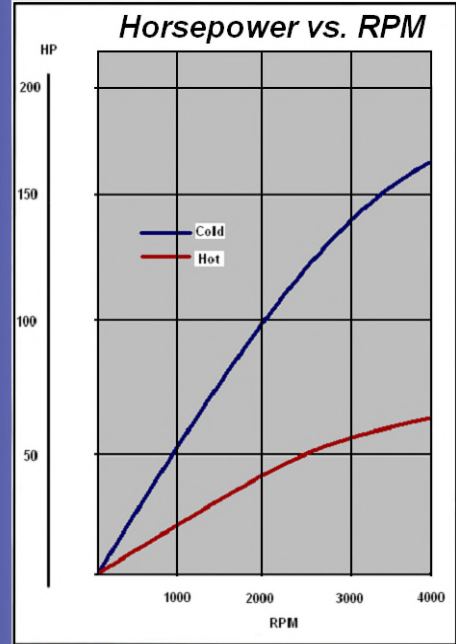
Single Brake Chart - ECB 50X
